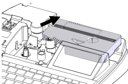
Removal of Printing Material cassette
