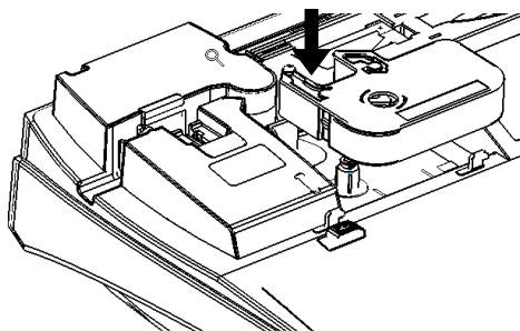
Installation of Ribbon
