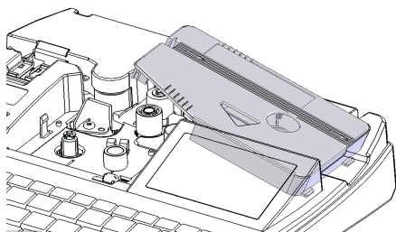
Installation of Label cassette
